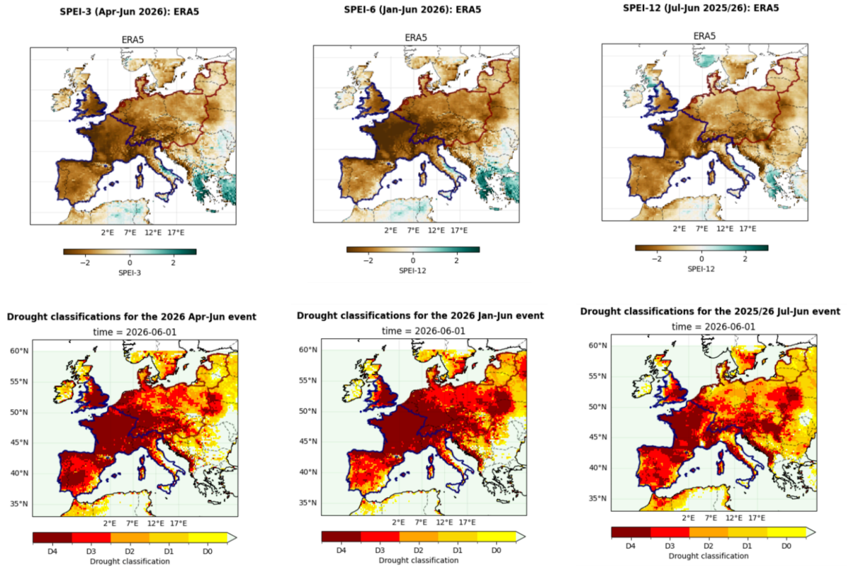
Figure 1.3 Top: Precipitation anomalies wrt 1991-2020 for 3-, 6- and 12-month accumulated precipitation ending in June 2026. Middle: SPEI maps for 3-, 6- and 12- month accumulation periods ending in June 2026 over the region 33-60°N,15°W-30°E. The Western Domain is highlighted in blue and the Eastern Domain is highlighted in red. Bottom: Drought classification maps categorised according to the US Drought Monitor (USDM) system. The categories are based on the n-month SPEI values in June 2026, calculated from ERA5 using the Hargreaves scheme for PET.
