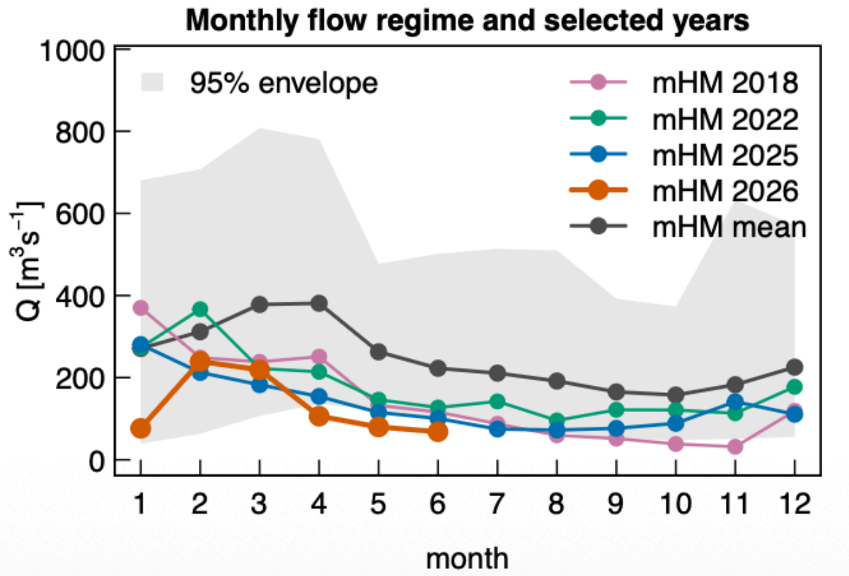
Figure 2.13: Monthly mean discharge of the Elbe River at Decin (GRDC ID: 6140400) near the Czech/German border, simulated by mHM forced with E-OBS meteorological data. Coloured lines show the monthly discharge for 2018, 2022, 2025 and January-June 2026. The dark-grey line shows the 1950-2025 climatological monthly mean, while the grey shading shows the 2.5th-97.5th percentile range for each calendar month over 1950-2025. The mean simulated discharge during April-June 2026 was the lowest for this period in the simulation record beginning in 1950.
